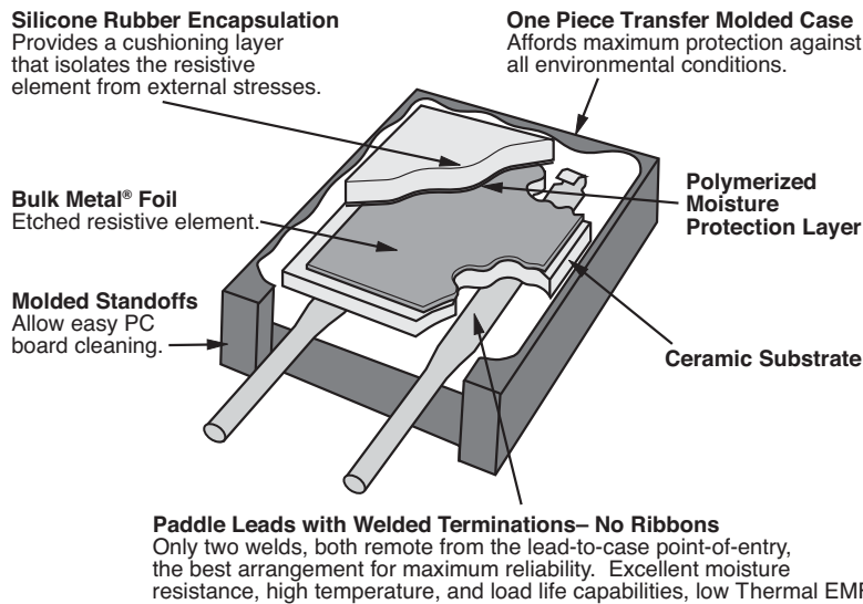
Figure 23. Ruggedized Construction
