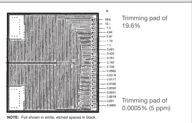
Figure 4. Vishay Foil Resistors S102C Resistor Element
