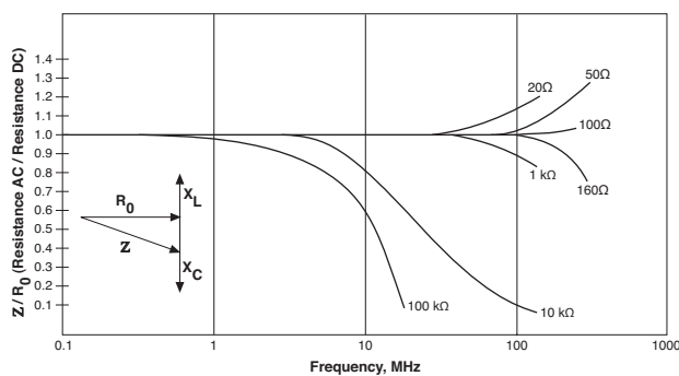
Figure 17. Effect of Operation at Frequency*
