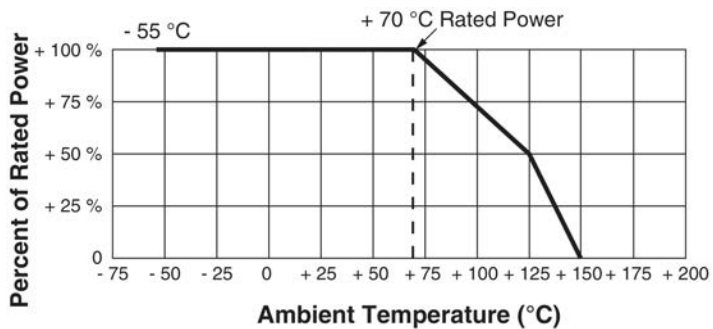
FIGURE 4 – POWER DERATING CURVE
